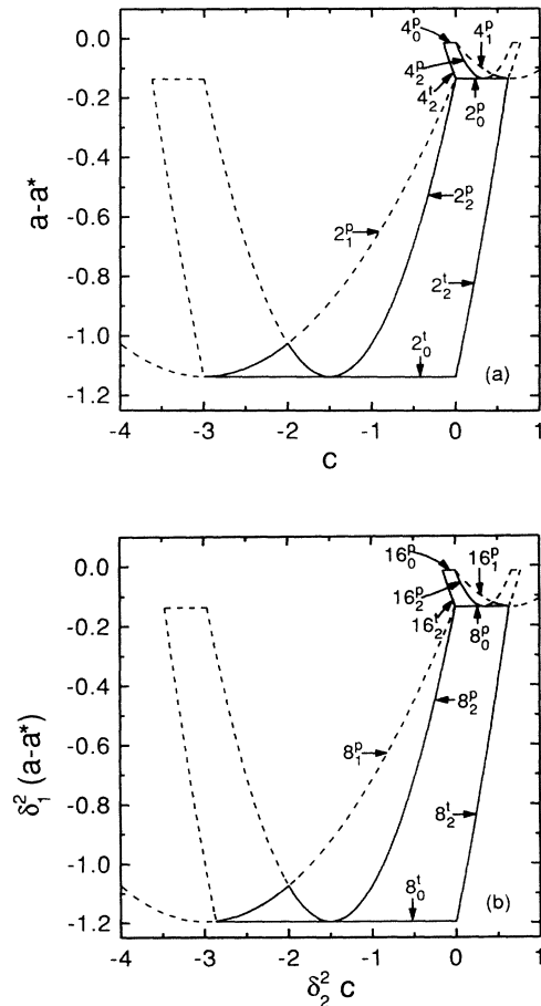
FIG. 2. Stable regions of the in-phase period- 2^n orbits of level n = 1, 2, 3, 4 in four linearly coupled maps with the nearest-neighbor coupling. The case of n = 1 and 2 (3 and 4) is shown in (a) [(b)]. Each stable region is bounded by its solid boundary curves. The period-doubling (tangent) bifurcation curve of the j mode of an in-phase orbit with period q is denoted by a symbol q_j^{p(t)} . The values of the scaling factors used in (b) are \delta_1 = 8.721 and \delta_2 = -4.404 .
